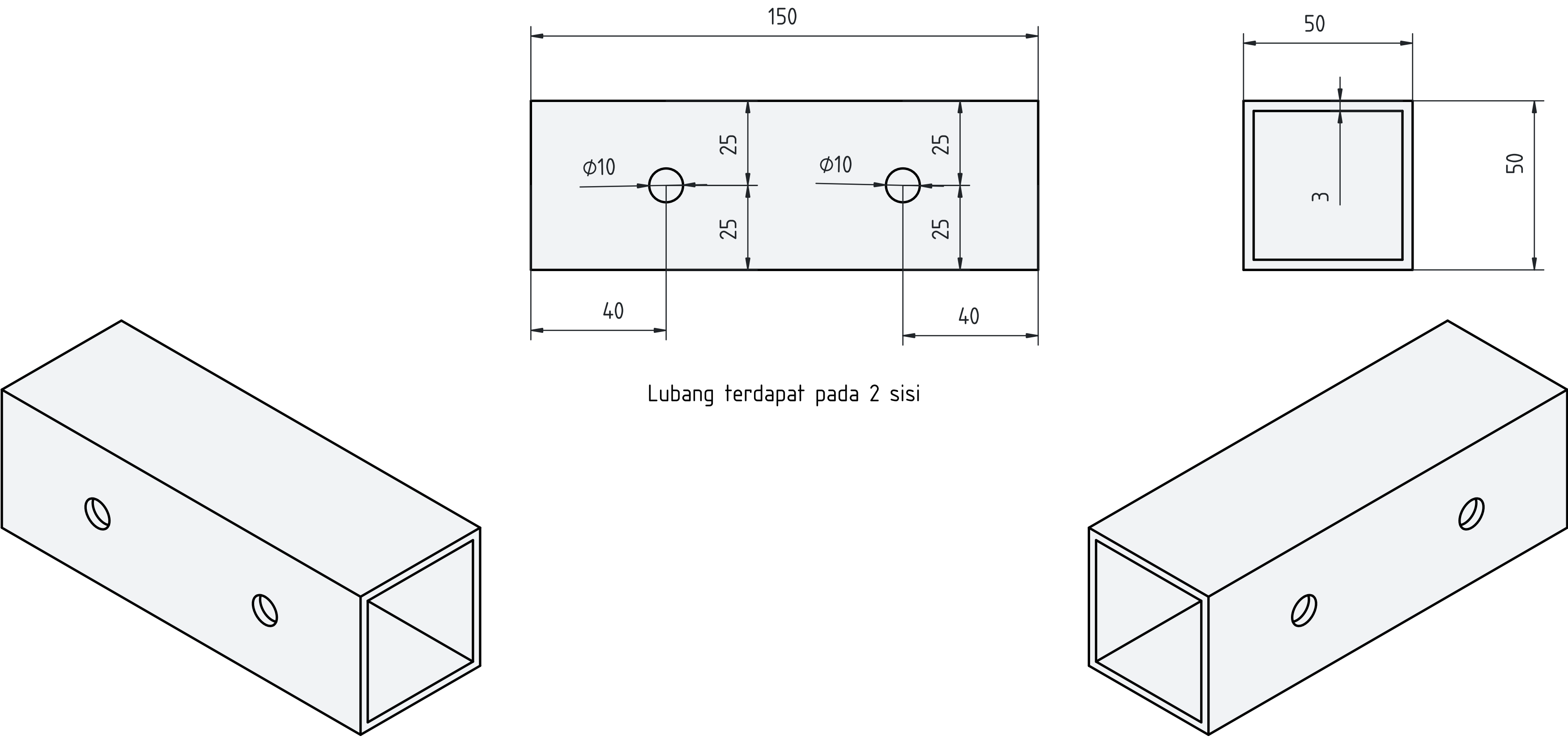
Besi Hollow Galvanis 50x50mm tebal 3mm
